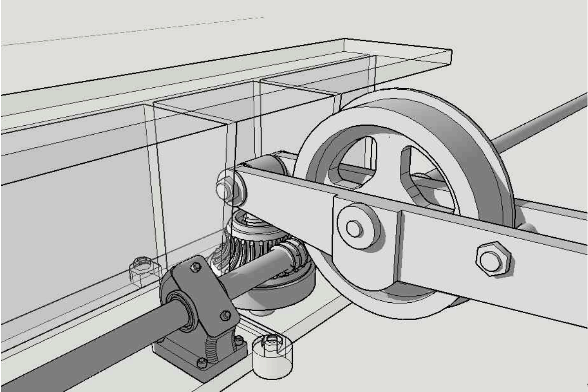
LIFING GEAR DOWN
